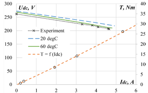
Fig. 8. Characteristics of electric generator.
